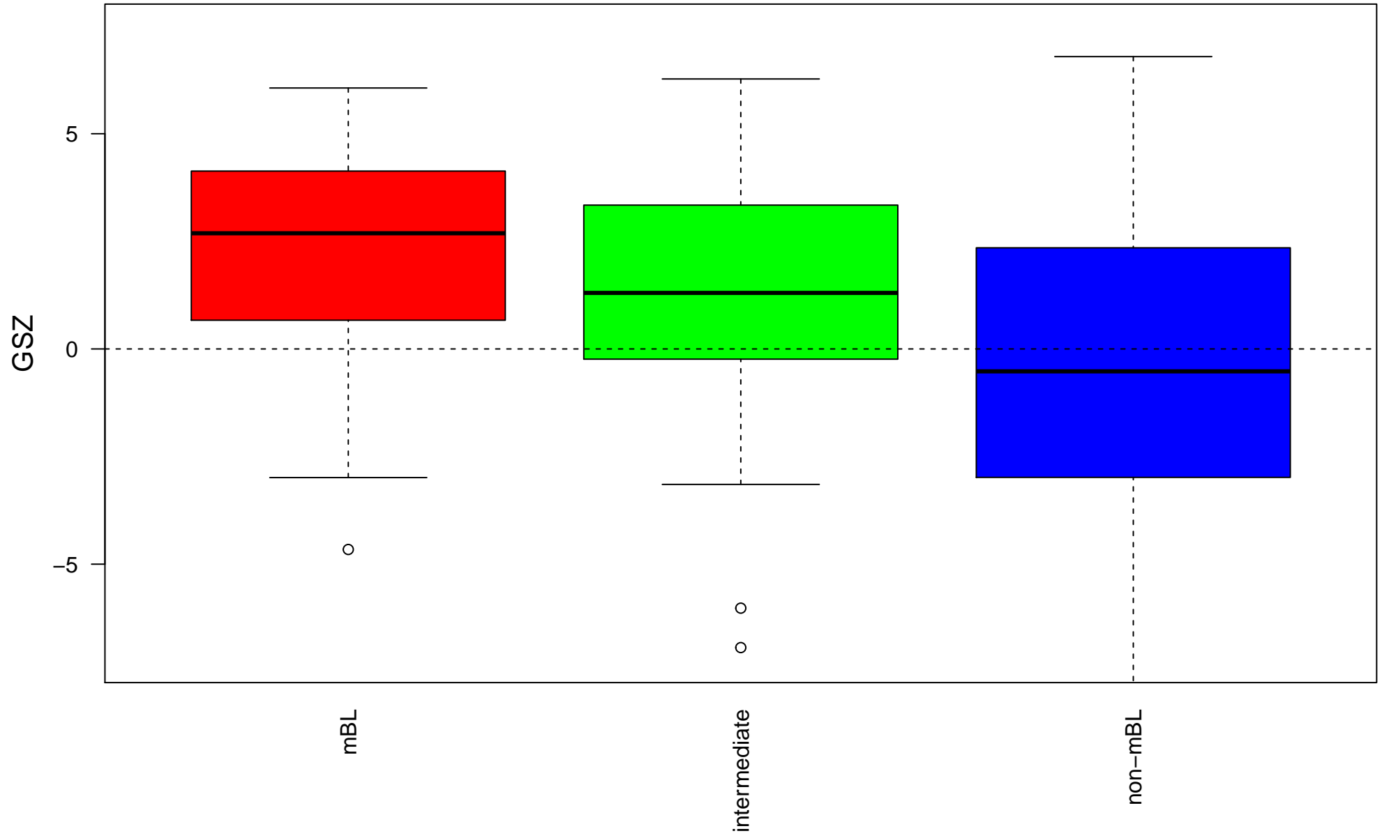
Monti_BCR_cluster
